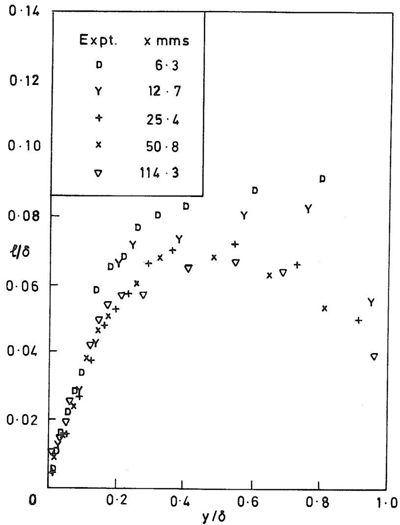
FIG. 45. Mixing length and eddy viscosity distributions ( M = 1.8 ; F = 0.00174 ).
