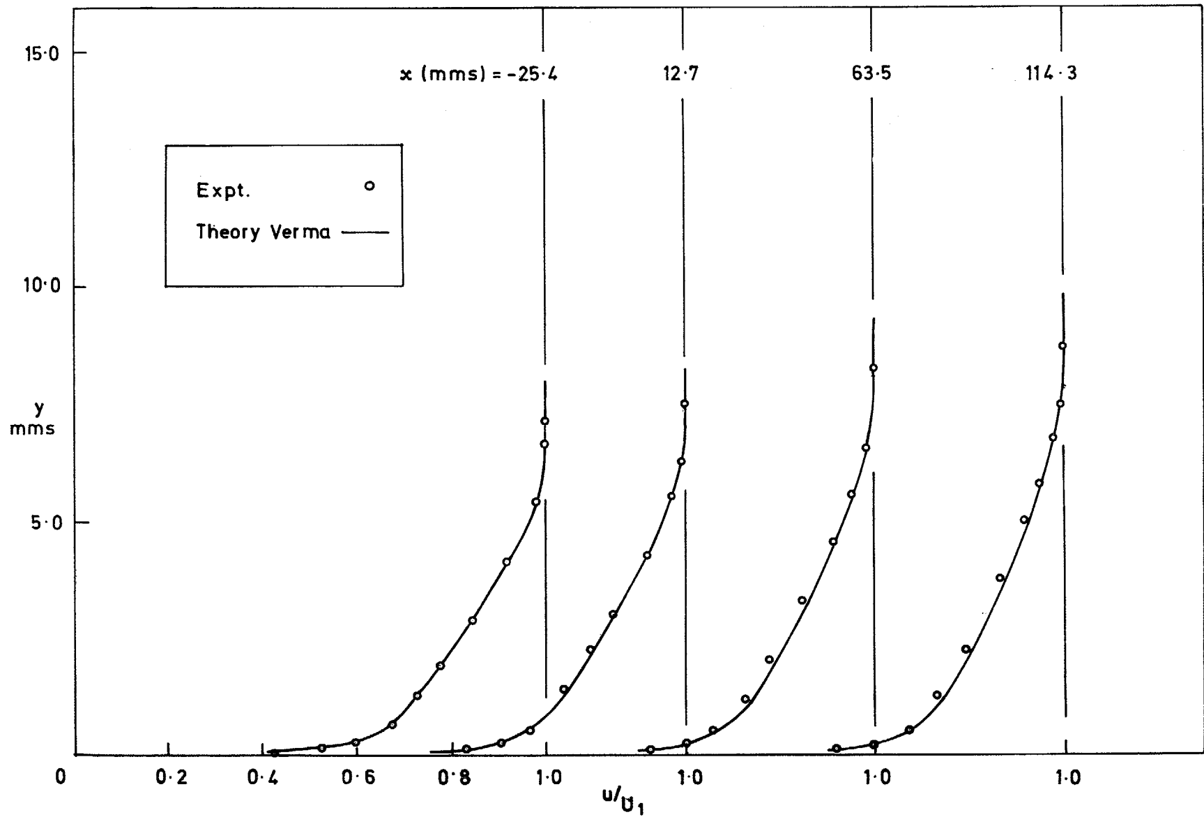
FIG. 14. Velocity profiles ( M = 3.6 ; F = 0 ).
