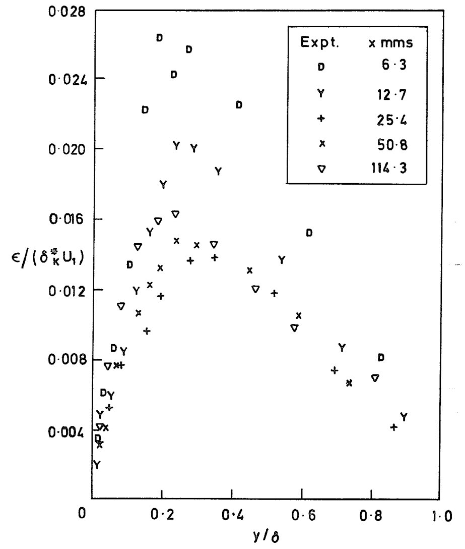
FIG. 47. Mixing length and eddy viscosity distributions ( M = 1.8; F = 0.00446 ).
