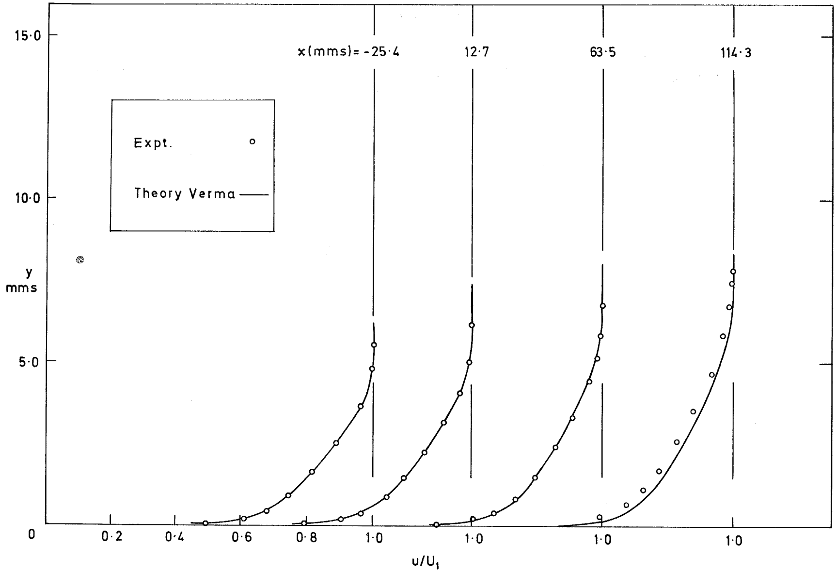
FIG. 10. Velocity profiles ( M = 1.8 ; F = 0 ).
