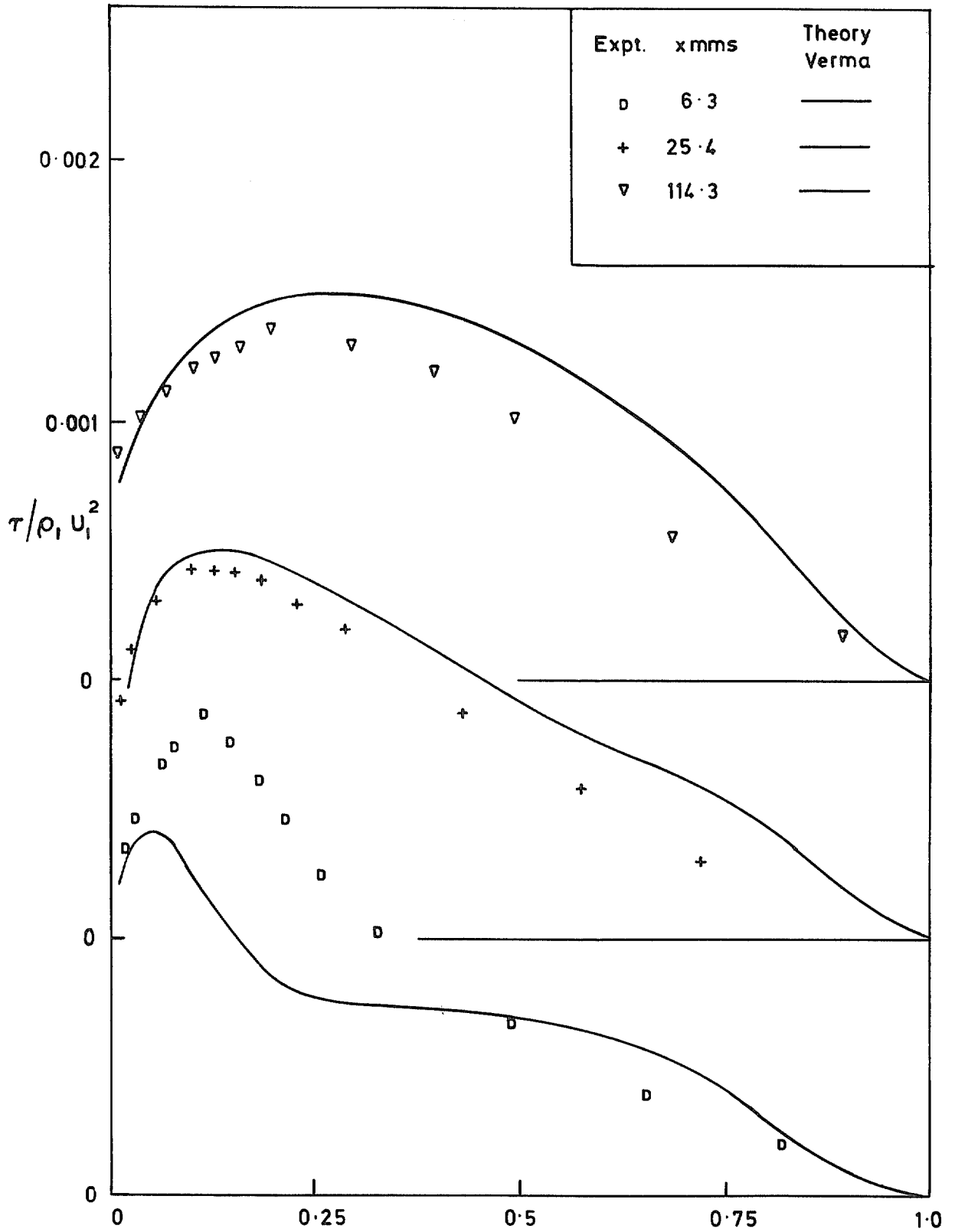
FIG. 43. Shear stress profiles ( M = 3.6; F = 0.00294 ).
