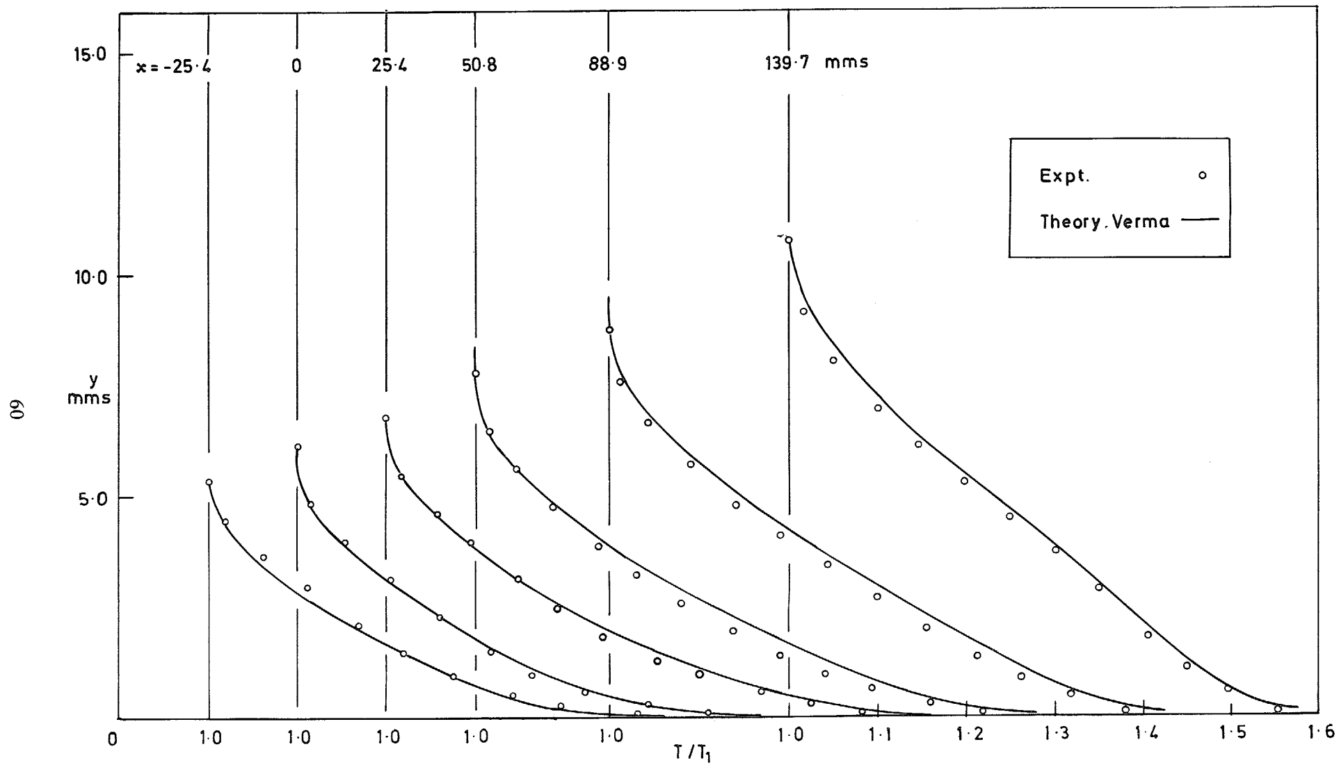
FIG. 13. Temperature profiles ( M = 1.8; F = 0.00446 ).
