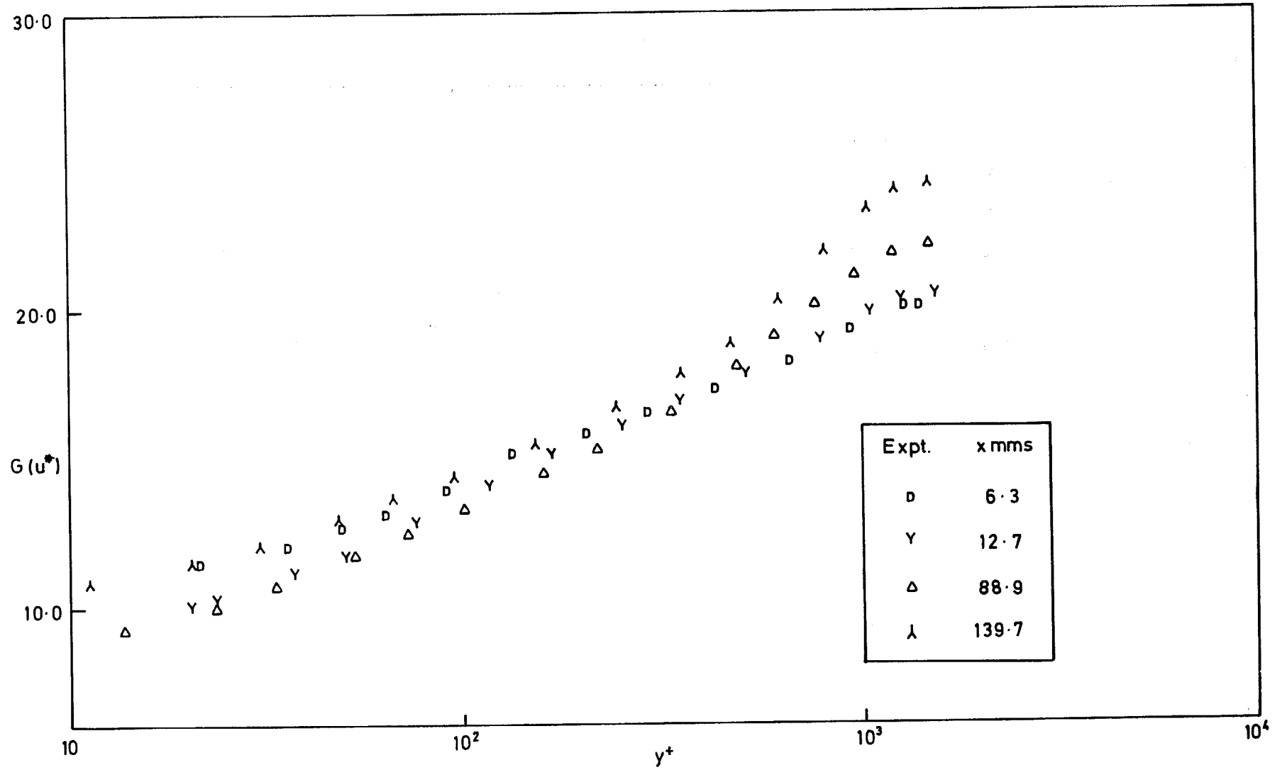
FIG. 40. G(u^*) vs \log(yU_\tau/\nu_w) ( M=1.8 ; F=0.00446 ).
