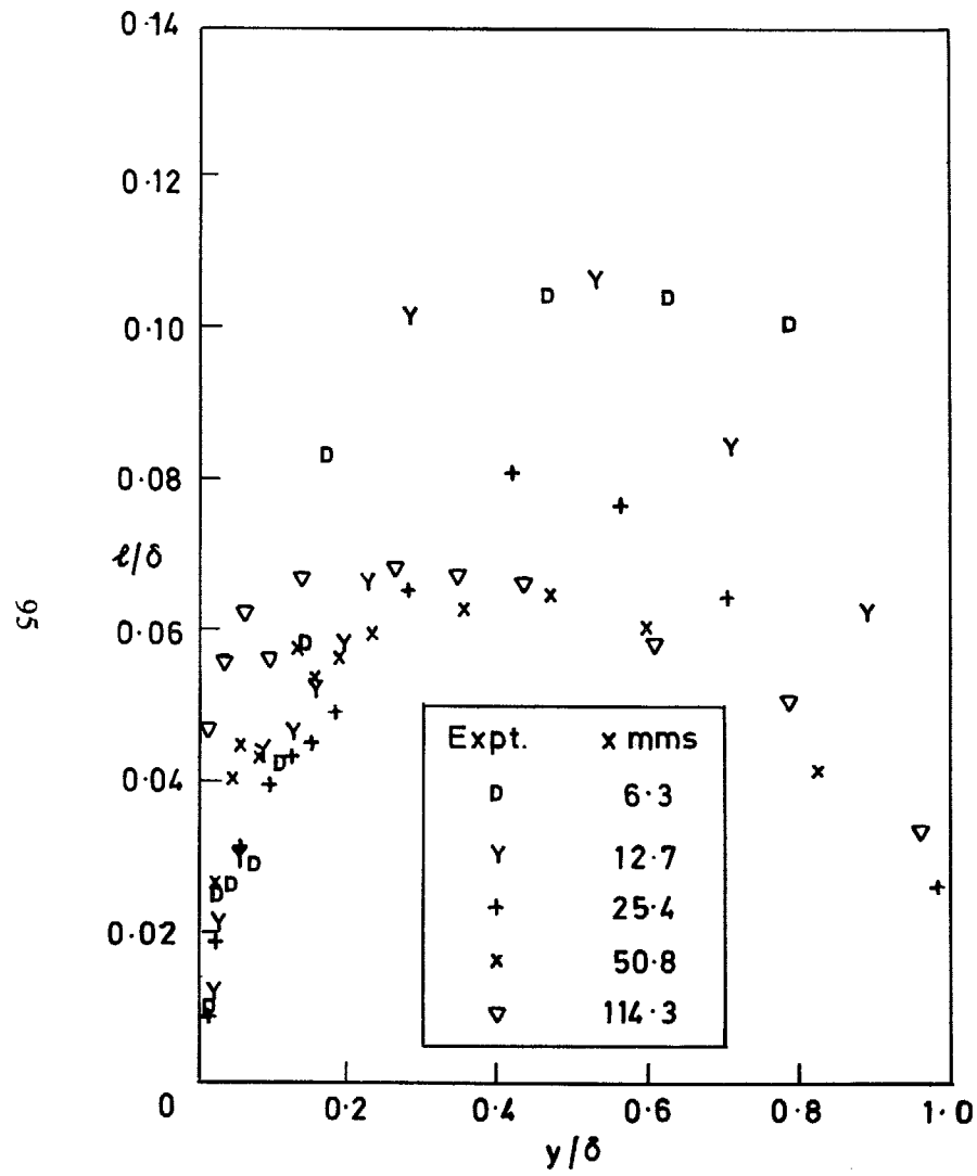
FIG. 48. Mixing length and eddy viscosity distributions ( M = 3.6 ; F = 0.00421 ).
