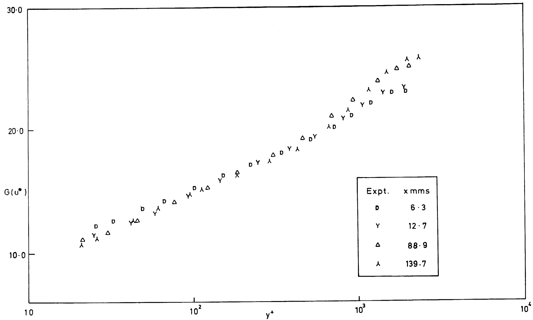
FIG. 38. G(u^*) vs (\log(yU_\tau/\nu_w)) ( M=1.8; F=0.00174 ).
