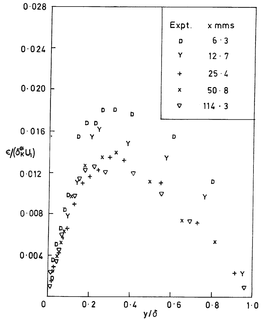
FIG. 45. Mixing length and eddy viscosity distributions ( M = 1.8 ; F = 0.00174 ).
