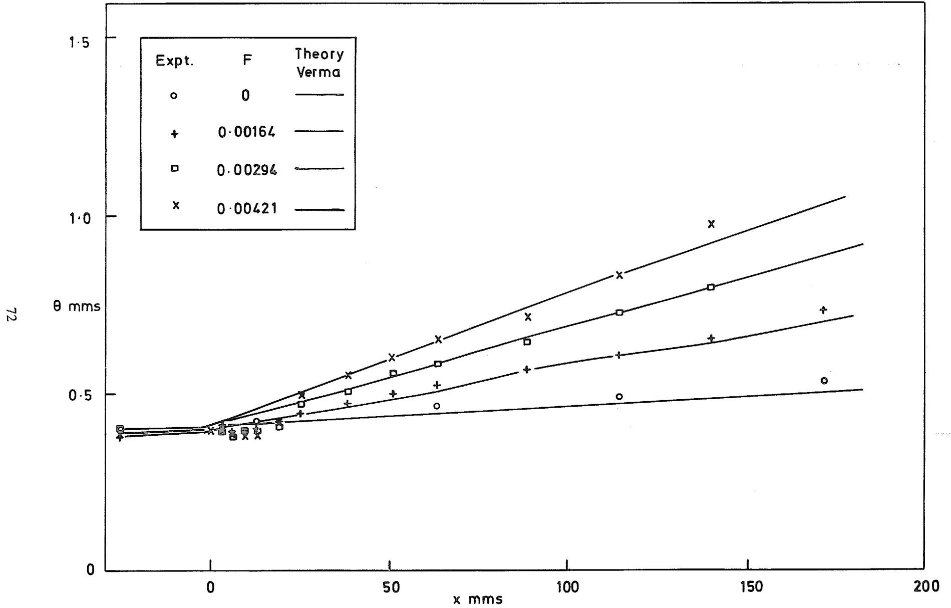
FIG. 25. Momentum thickness development ( M = 3.6 ).
