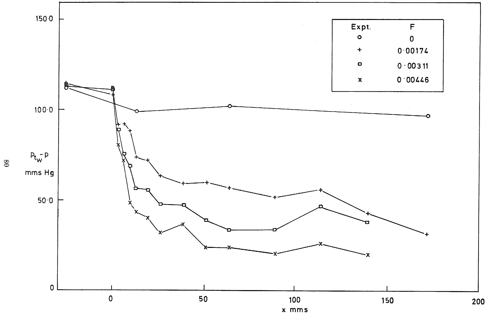
FIG. 33. Variation of dynamic pressure at the wall ( M = 1.8 ).
