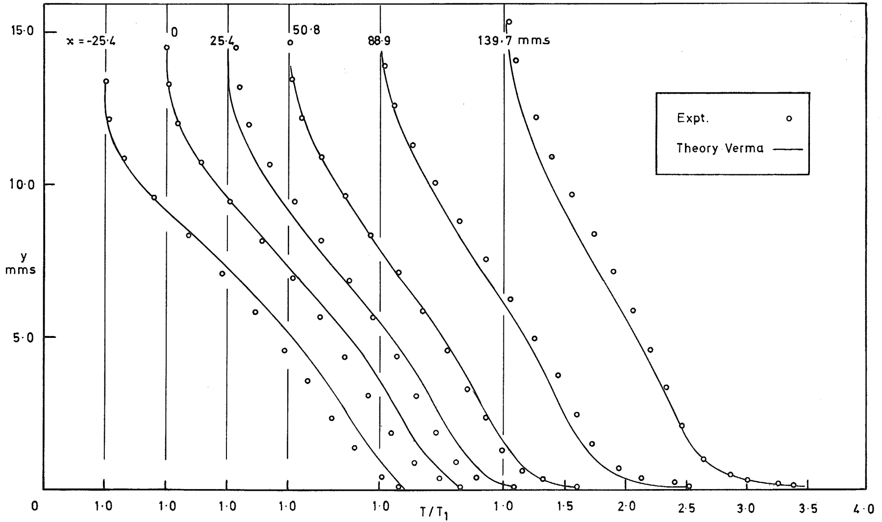
FIG. 21. Temperature profiles ( M = 3.6 ; F = 0.00294 porous-solid).
