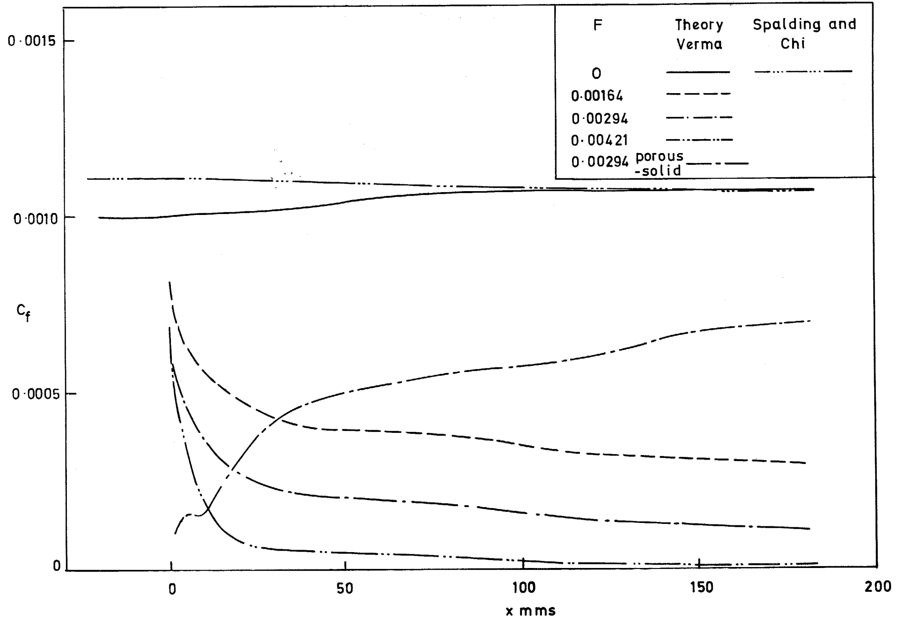
FIG. 34. Theoretical skin friction development ( M = 3.6 ).
