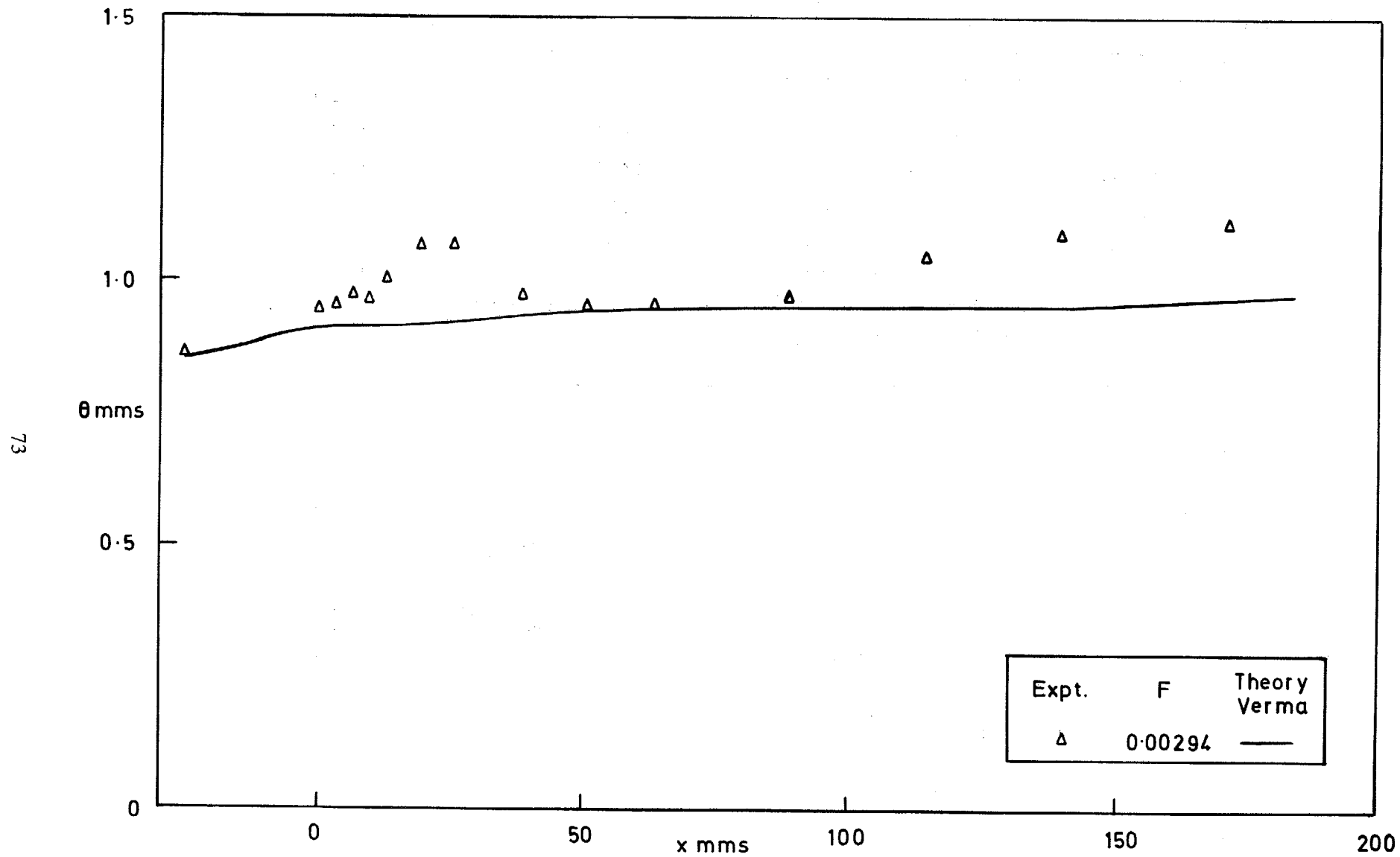
FIG. 26. Momentum thickness development ( M = 3.6 porous-solid).
