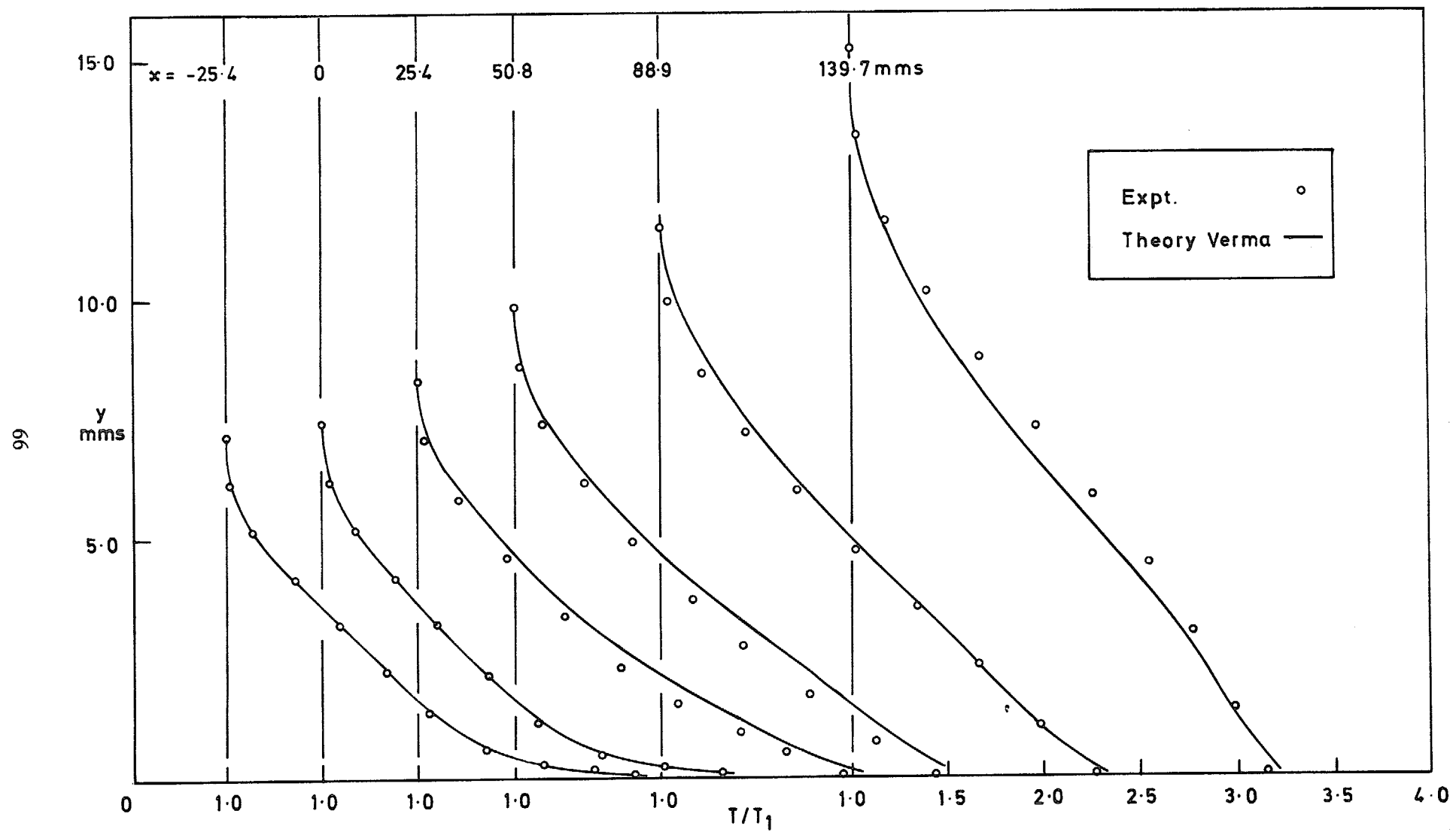
FIG. 19. Temperature profiles ( M = 3.6 ; F = 0.00421 ).
