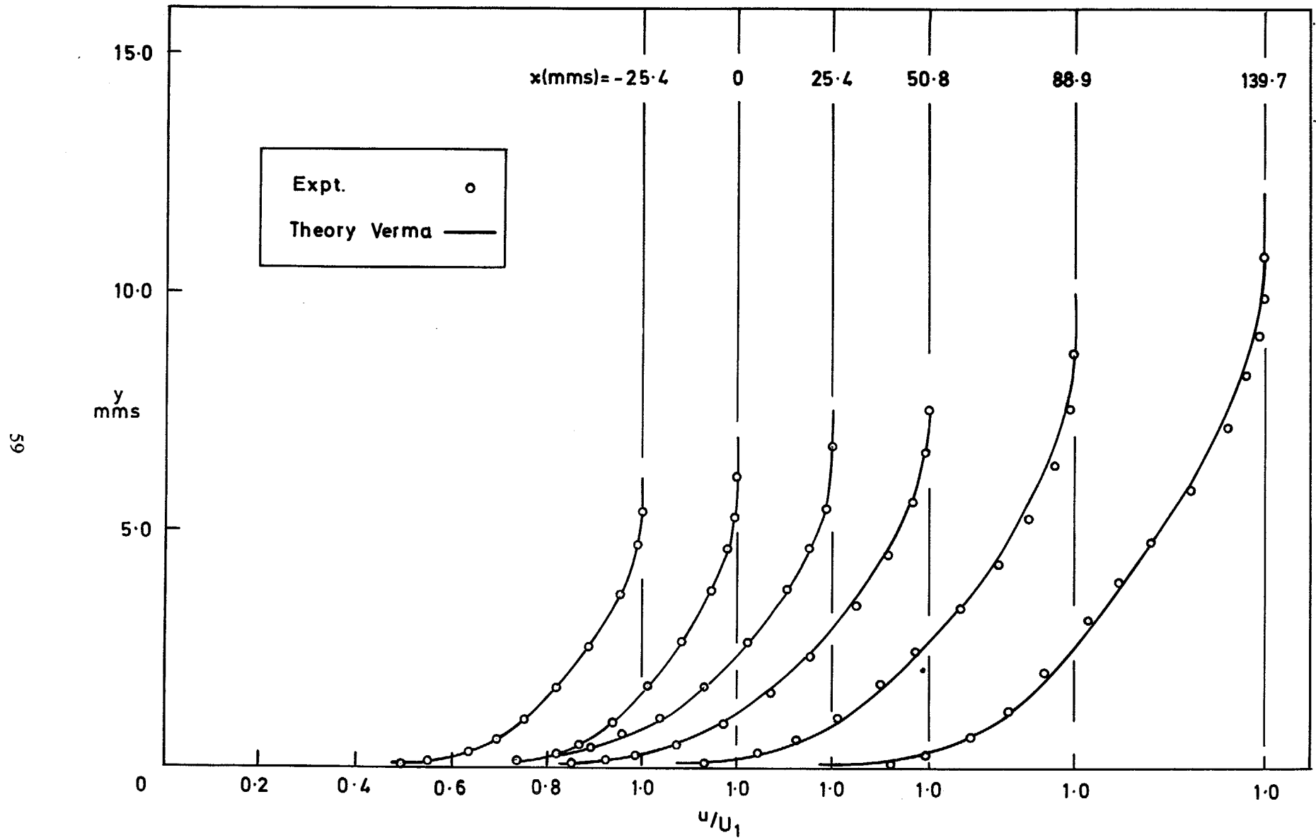
FIG. 12. Velocity profiles ( M = 1.8 ; F = 0.00446 ).
