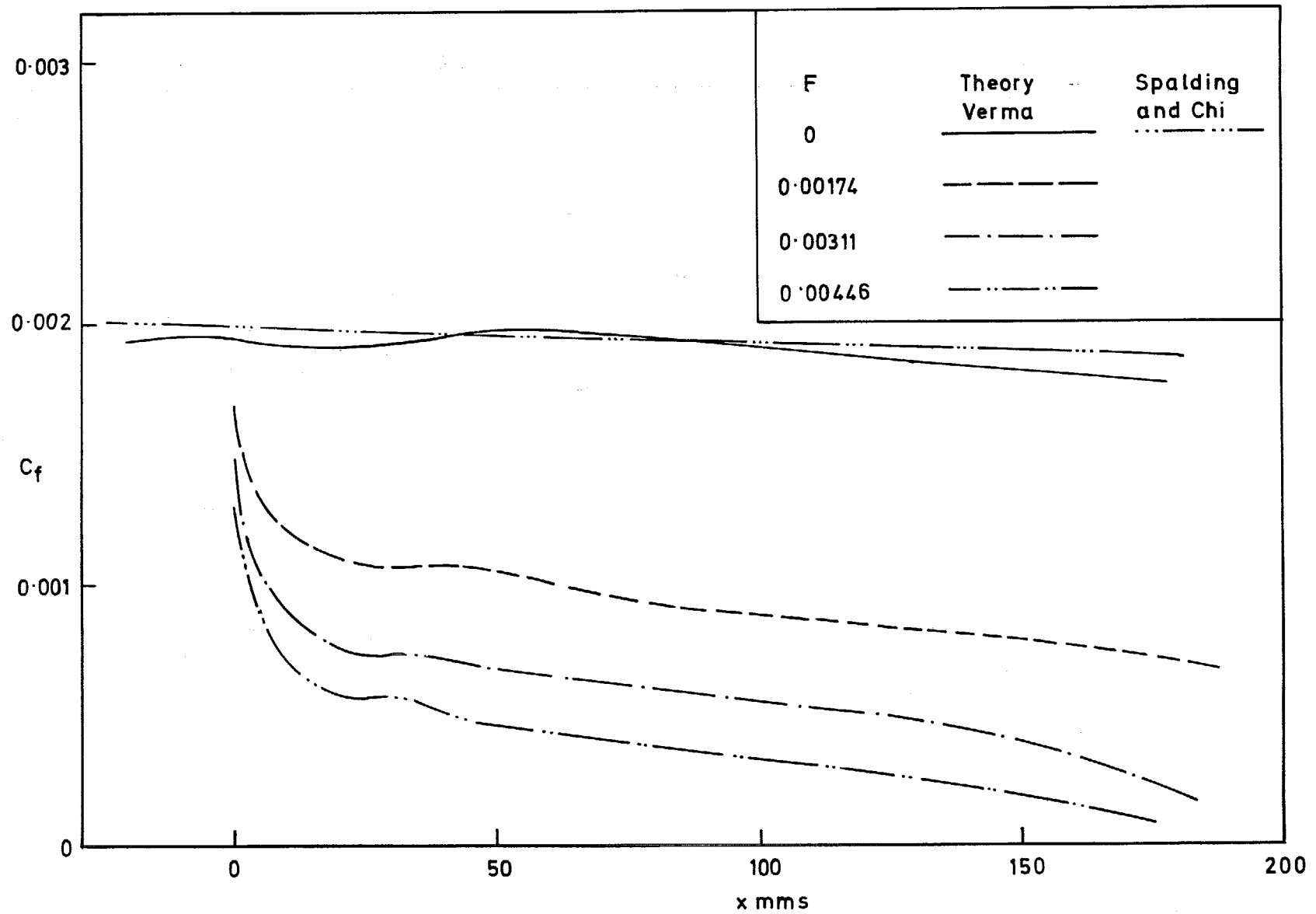
FIG. 32. Theoretical skin friction development ( M = 1.8 ).
