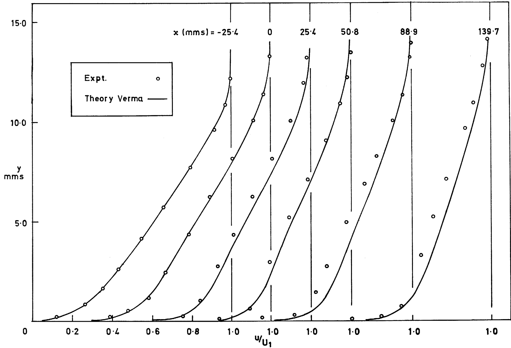
FIG. 20. Velocity profiles ( M = 3.6 ; F = 0.00294 porous-solid).
