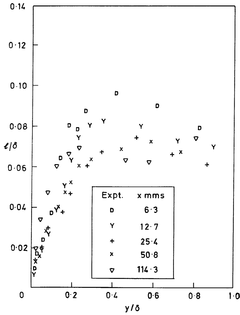
FIG. 47. Mixing length and eddy viscosity distributions ( M = 1.8; F = 0.00446 ).
