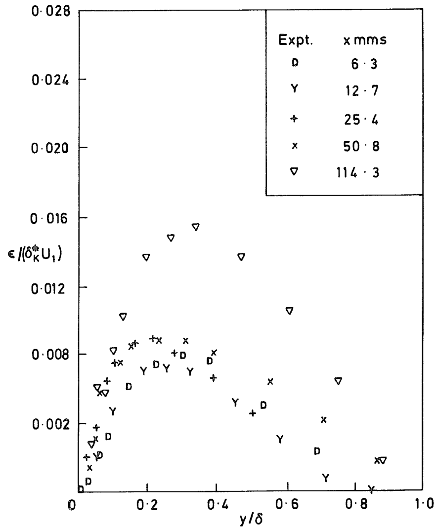
FIG. 49. Mixing length and eddy viscosity distributions ( M = 3.6 ; F = 0.00294 porous-solid).
