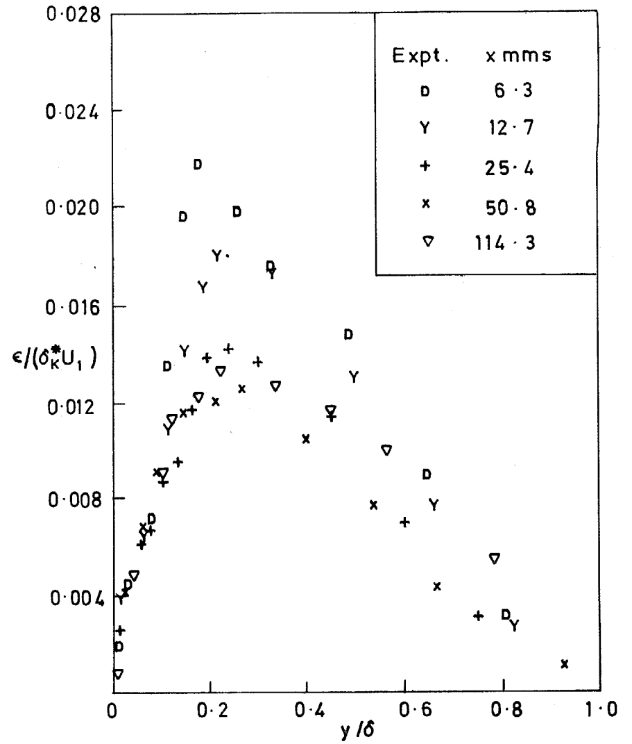
FIG. 46. Mixing length and eddy viscosity distributions ( M = 3.6 ; F = 0.00164 ).
