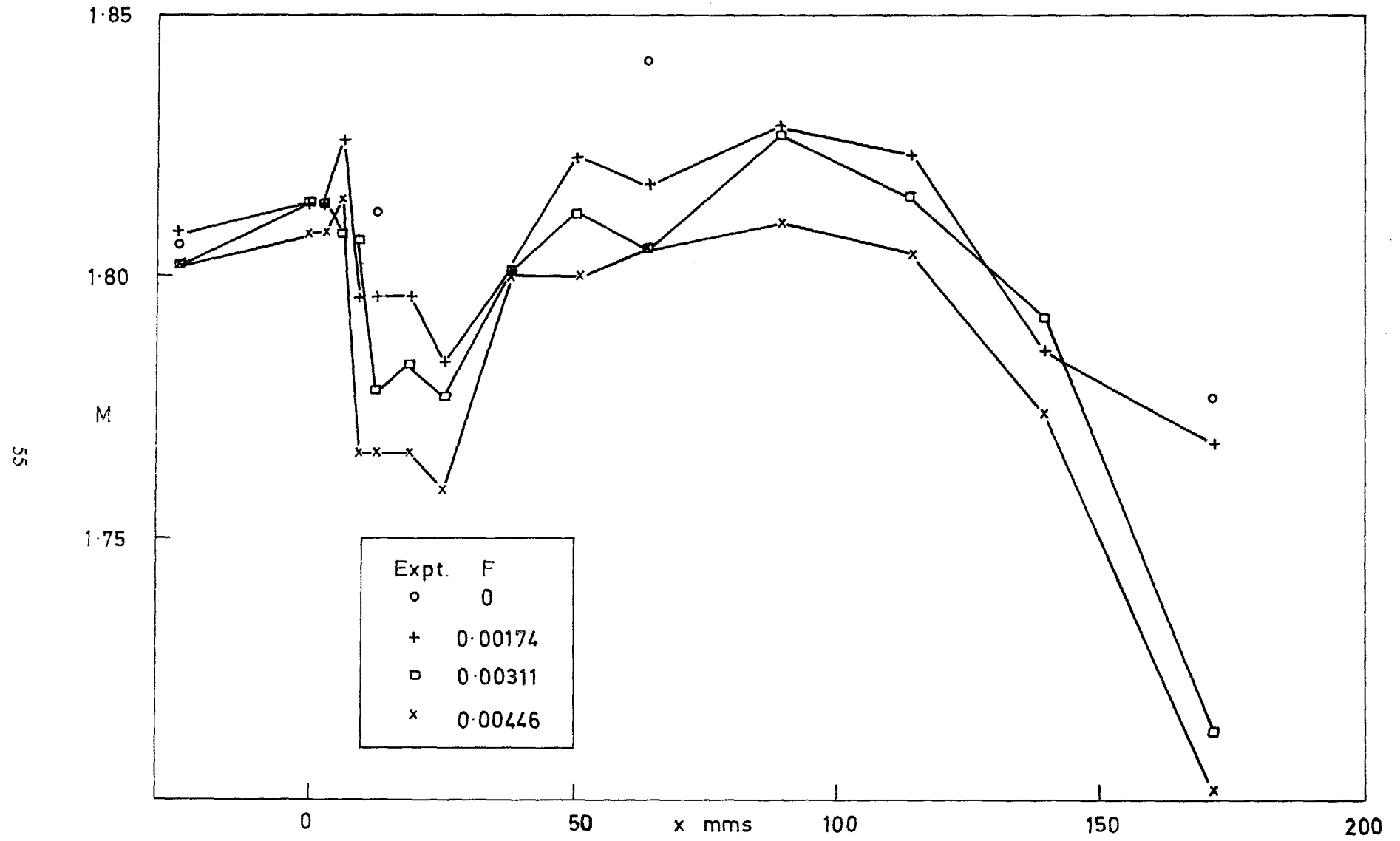
FIG. 8. Mach number distribution.
