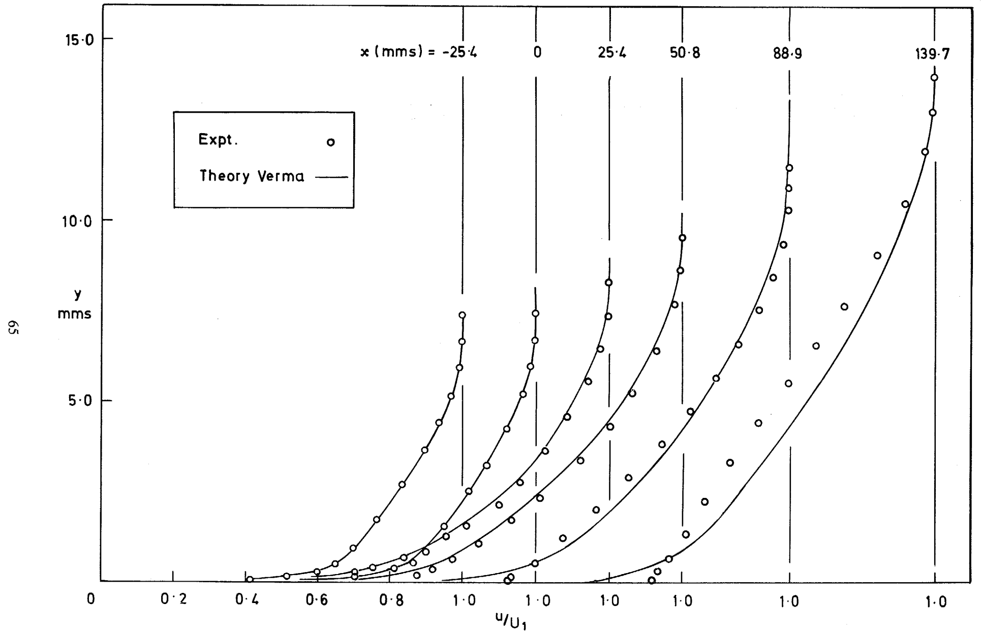
FIG. 18. Velocity profiles ( M = 3.6 ; F = 0.00421 ).
