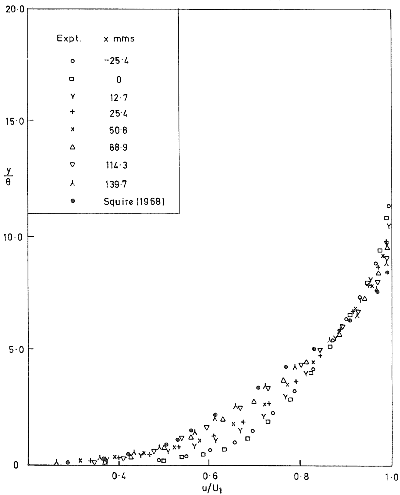
FIG. 29. y/\theta vs u/U_1 ( M = 1.8 ; F = 0.00311 ).
