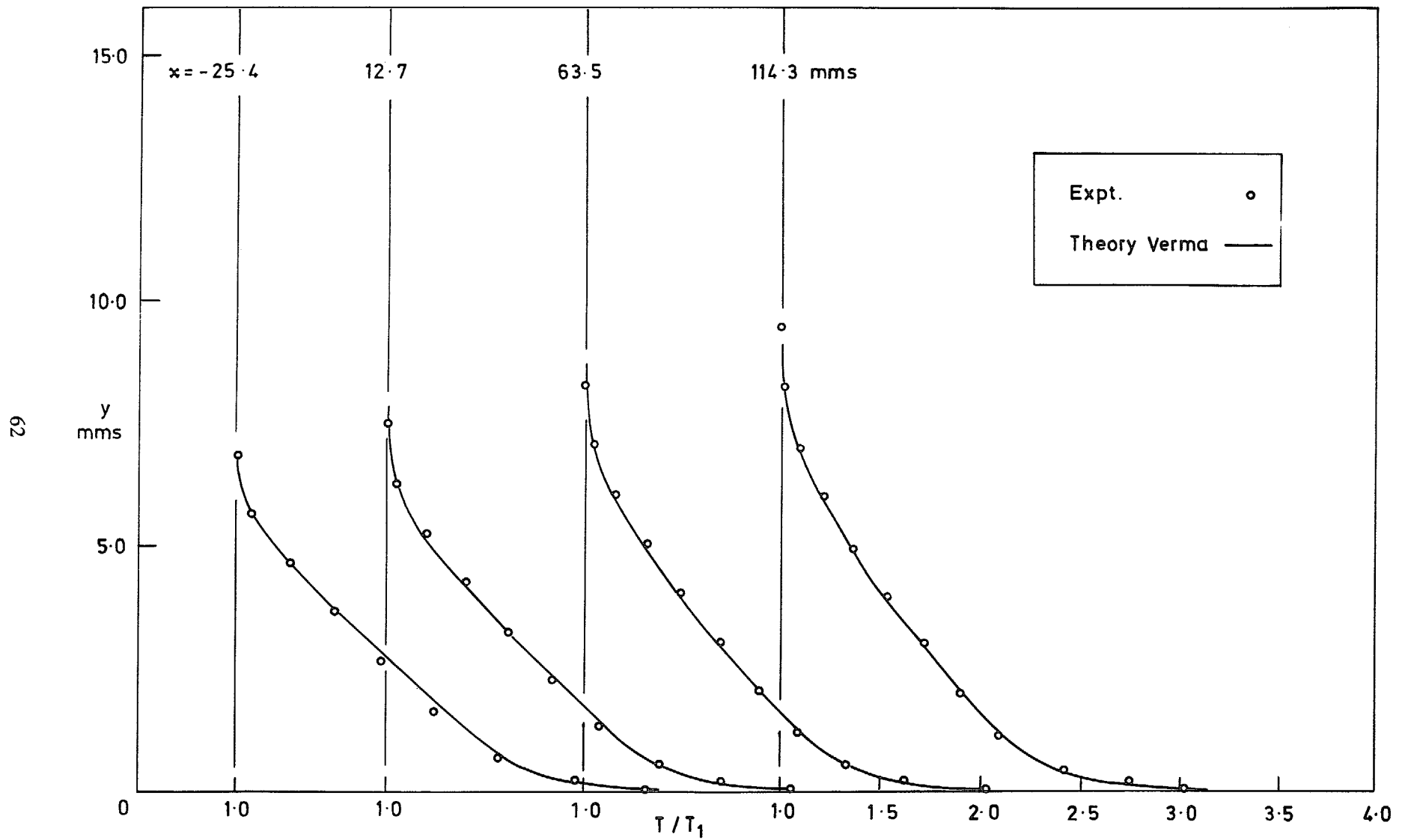
FIG. 15. Temperature profiles ( M = 3.6; F = 0 ).
