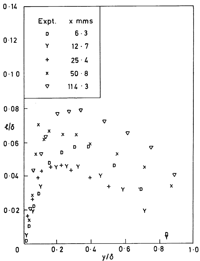
FIG. 49. Mixing length and eddy viscosity distributions ( M = 3.6 ; F = 0.00294 porous-solid).
