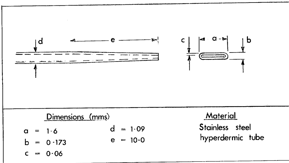
(a) Dimensions of the pitot probe
