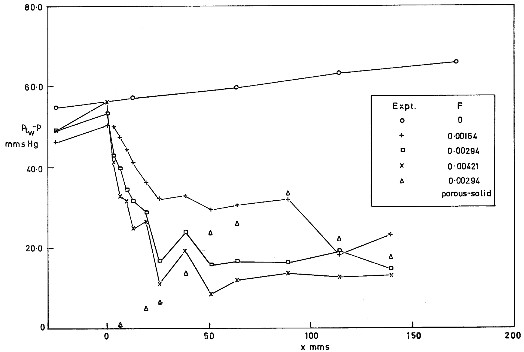
FIG. 35. Variation of dynamic pressure at the wall ( M = 3.6 ).
