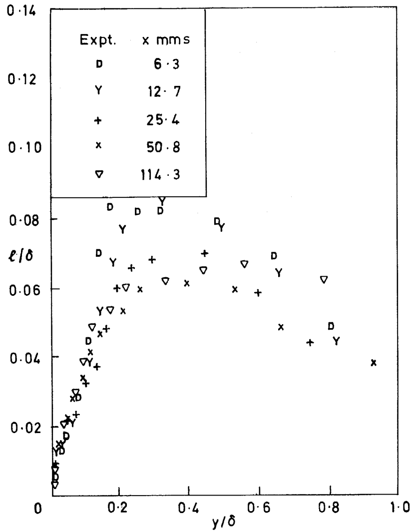
FIG. 46. Mixing length and eddy viscosity distributions ( M = 3.6 ; F = 0.00164 ).
