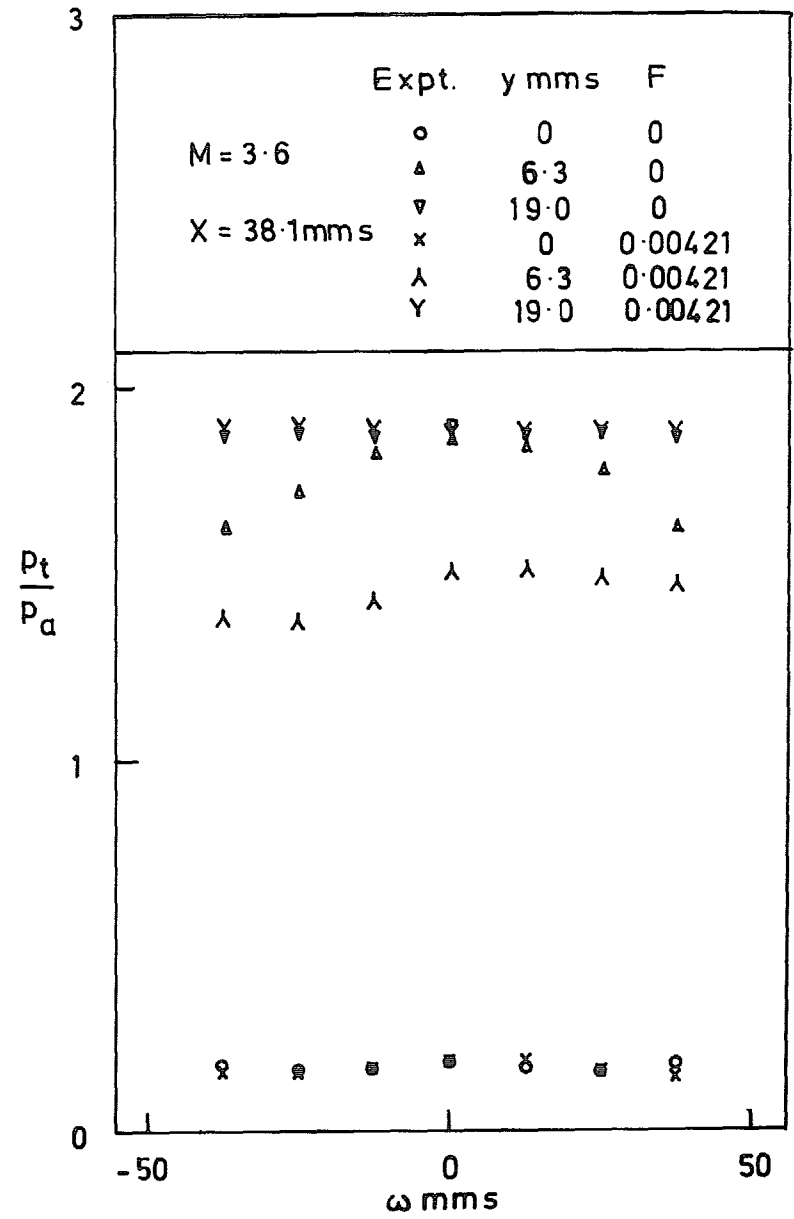
FIG. 7. Total pressure variation across plate.
