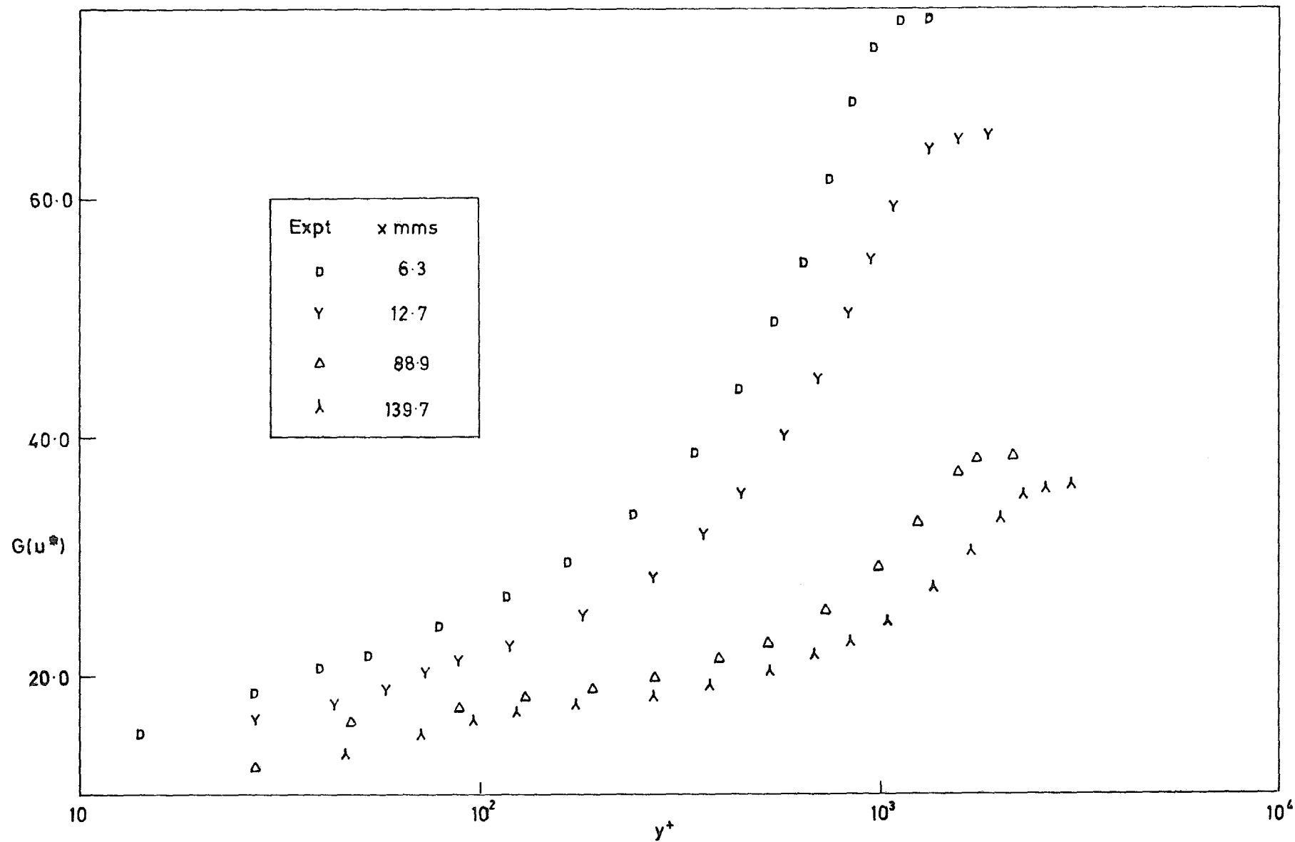
FIG. 37. G(u^*) vs \log(yU_\tau/\nu_w) ( M = 3.6 ; F = 0.00294 porous-solid).
