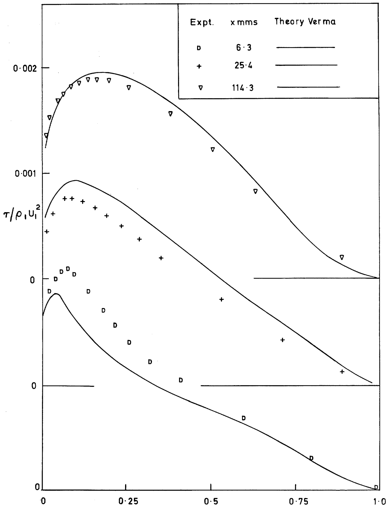
FIG. 42. Shear stress profiles ( M = 1.8; F = 0.00311 ).
