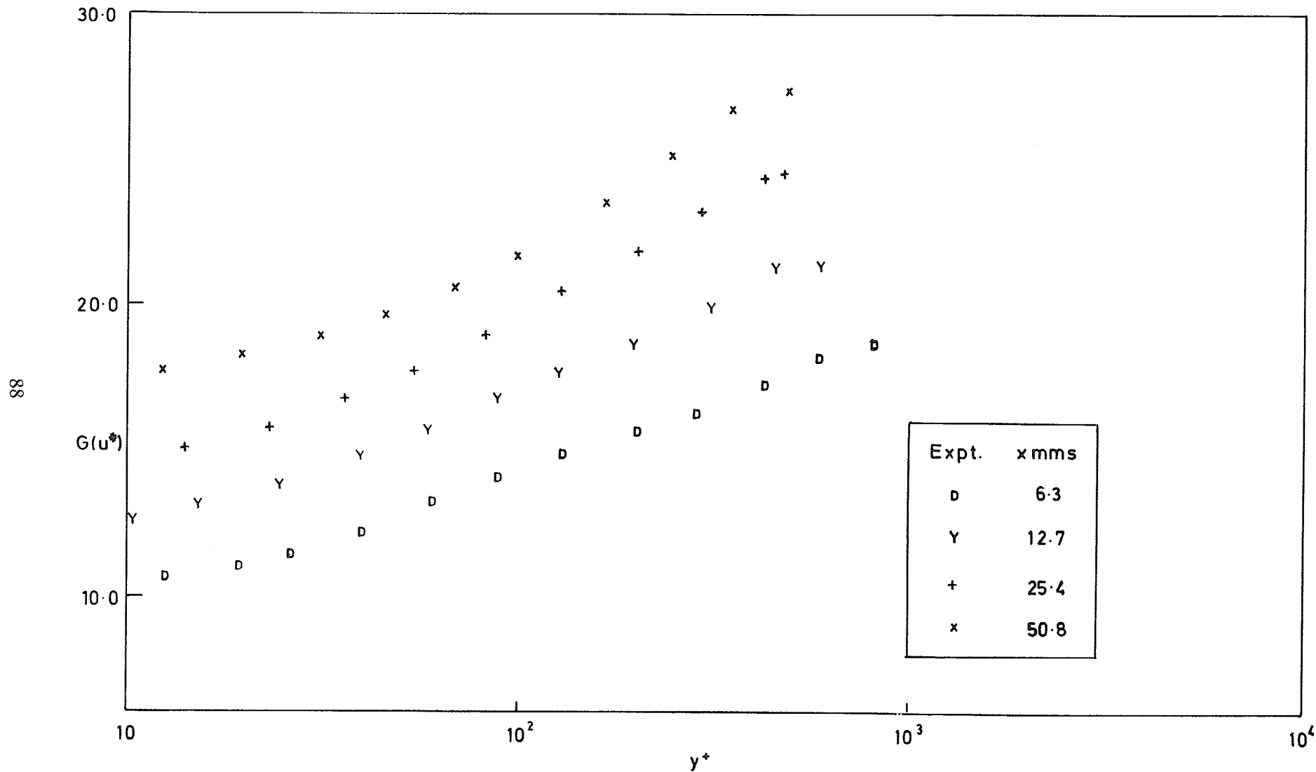
FIG. 41. G(u^*) vs \log(yU_\tau/\nu_w) ( M=3.6; F=0.00421 ).
