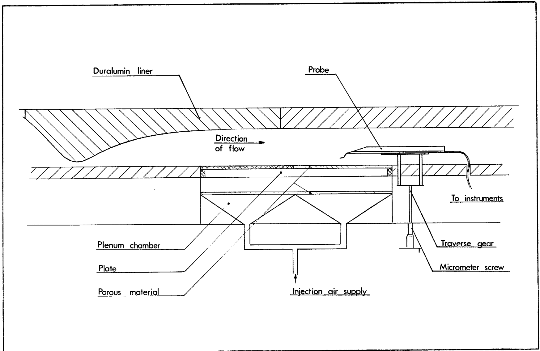
FIG. 2. Sketch of the working section.
