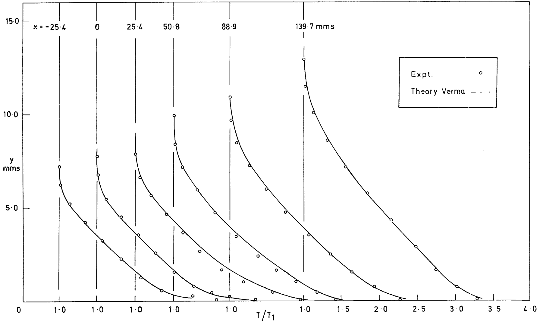
FIG. 17. Temperature profiles ( M = 3.6 ; F = 0.00294 ).
