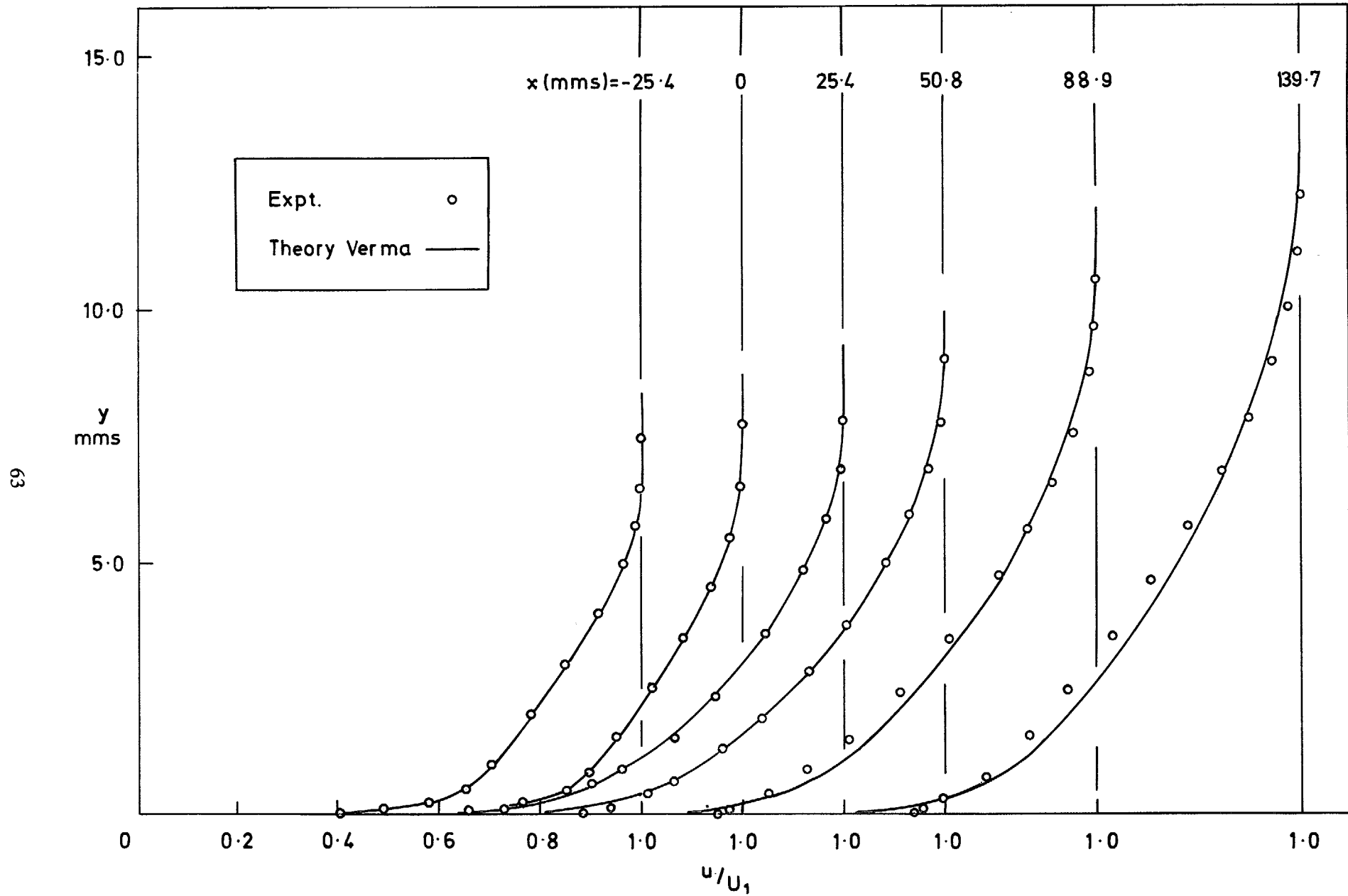
FIG. 16. Velocity profiles ( M = 3.6 ; F = 0.00294 ).
