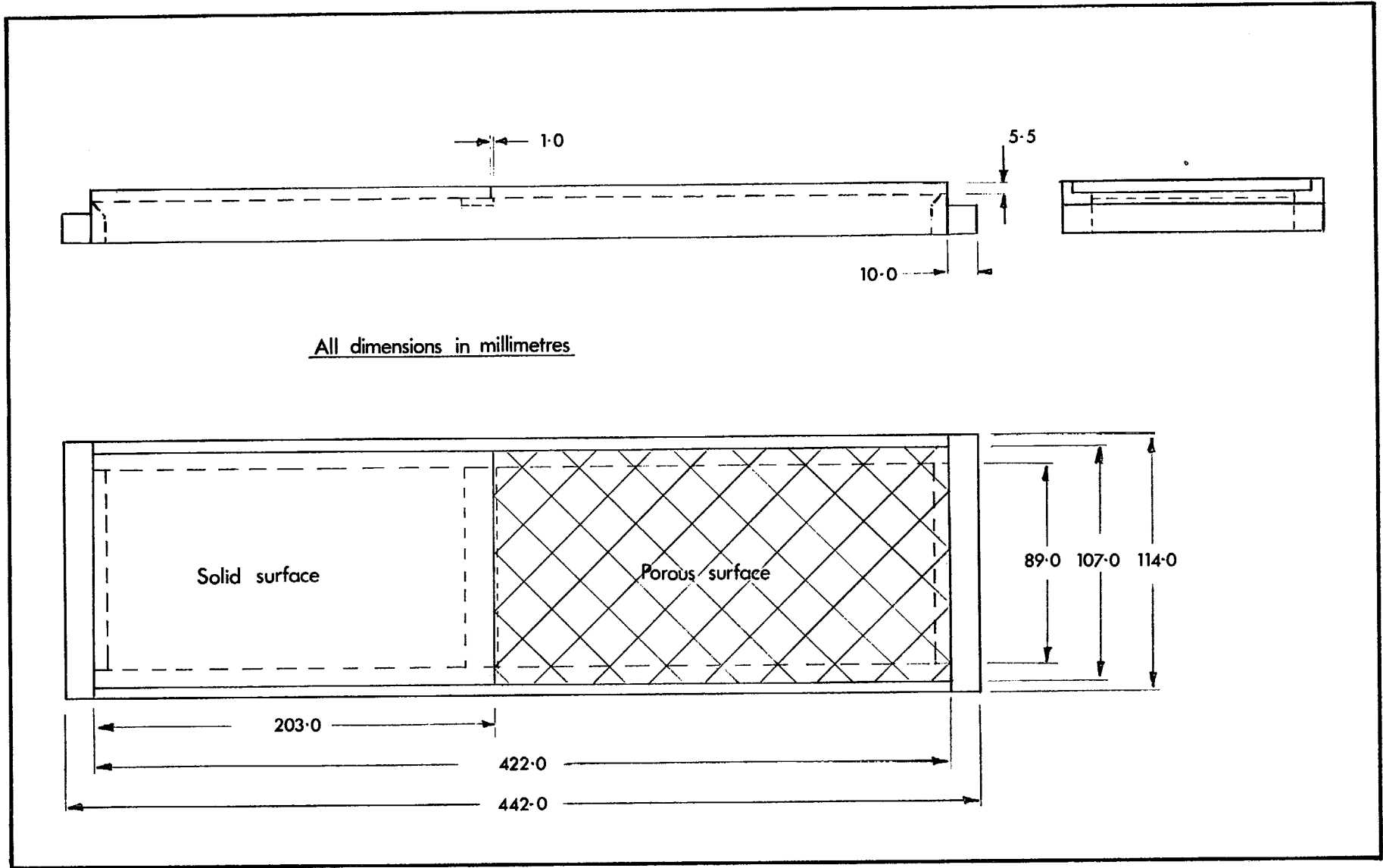
FIG. 4. Dimensions of the plate.
