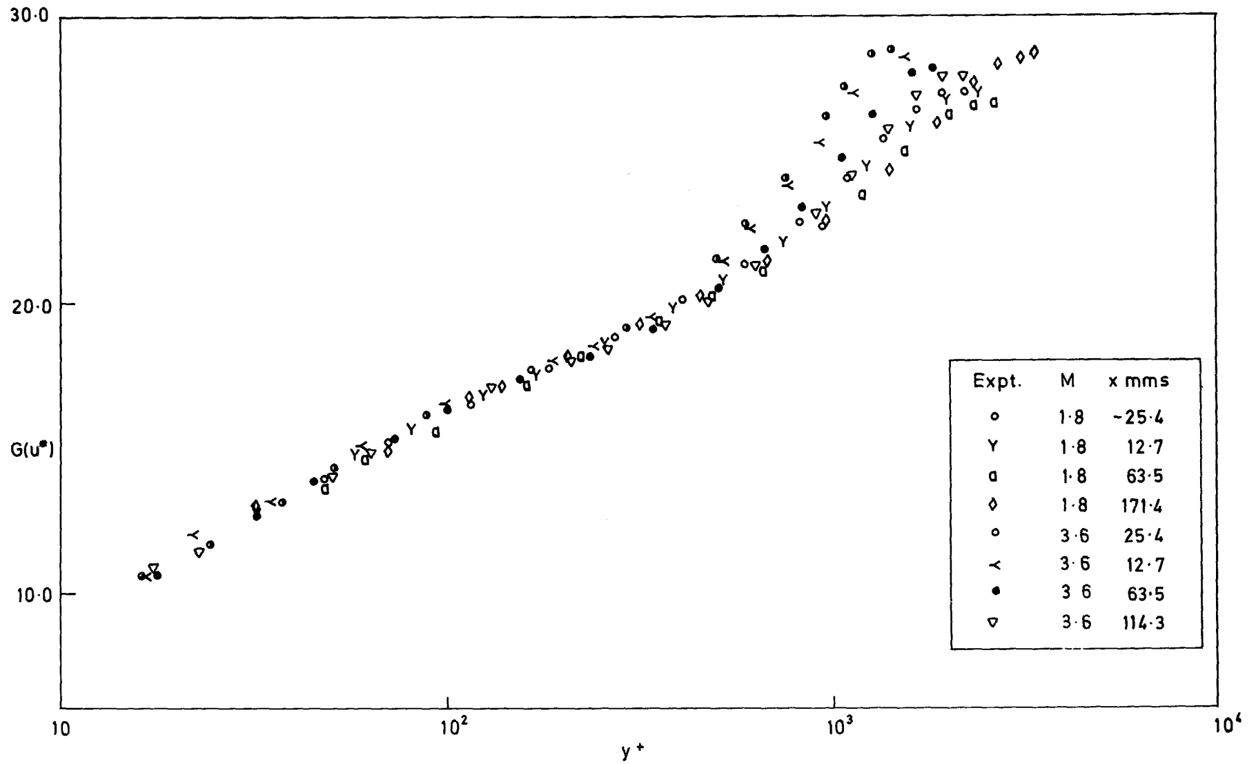
FIG. 36. G(u^*) vs \log(yU_\tau/\nu_w) ( M = 1.8; 3.6; F = 0 ).
