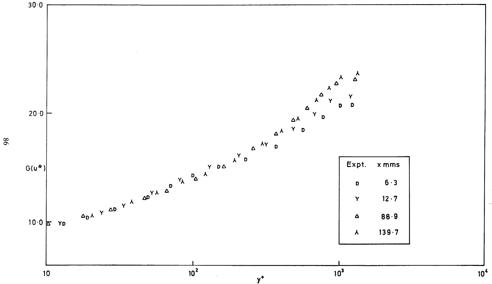
FIG. 39. G(u^*) vs \log(yU_\tau/\nu_w) ( M = 3.6 ; F = 0.00164 ).
