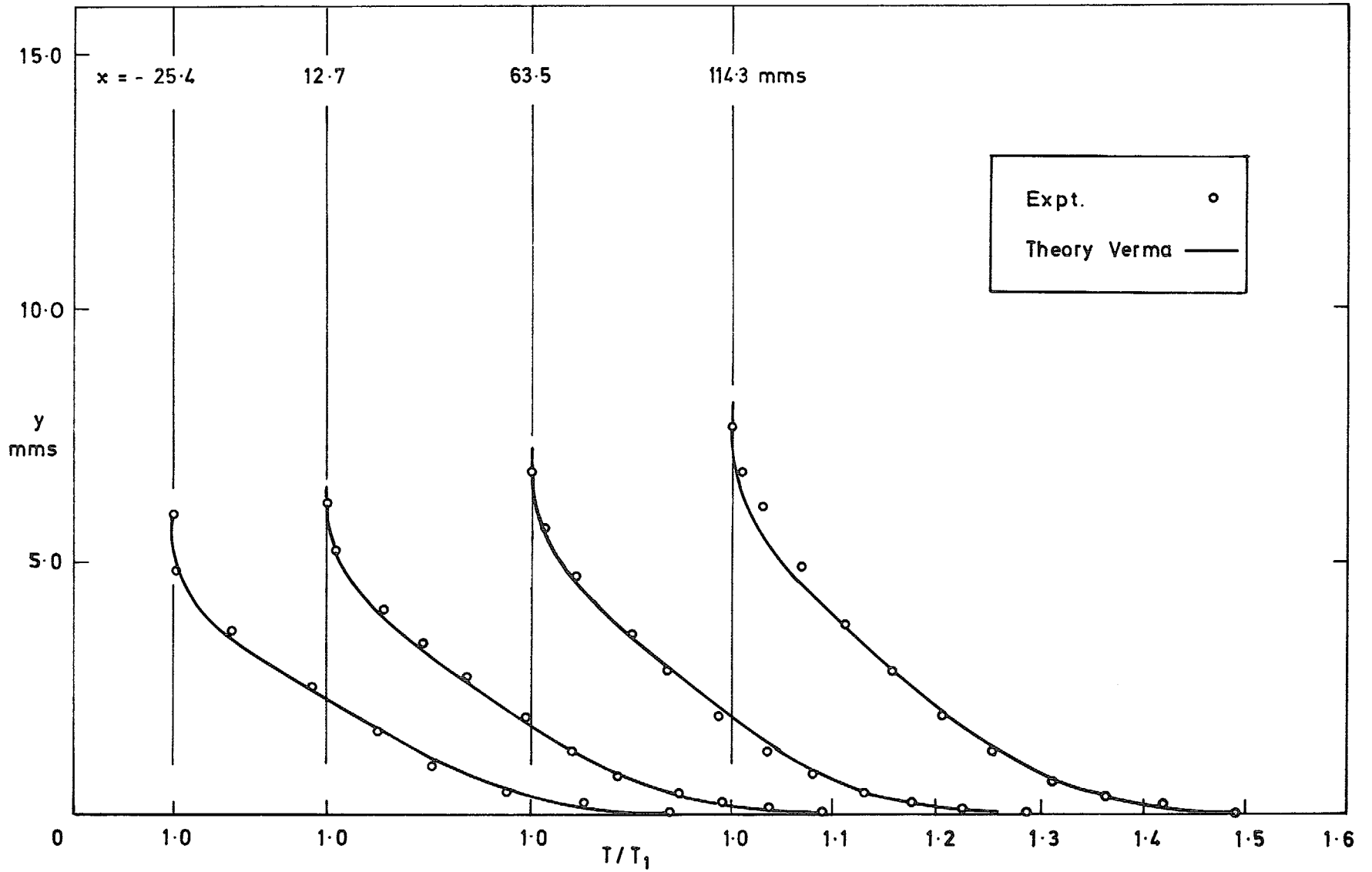
FIG. 11. Temperature profiles ( M = 1.8 ; F = 0 ).
