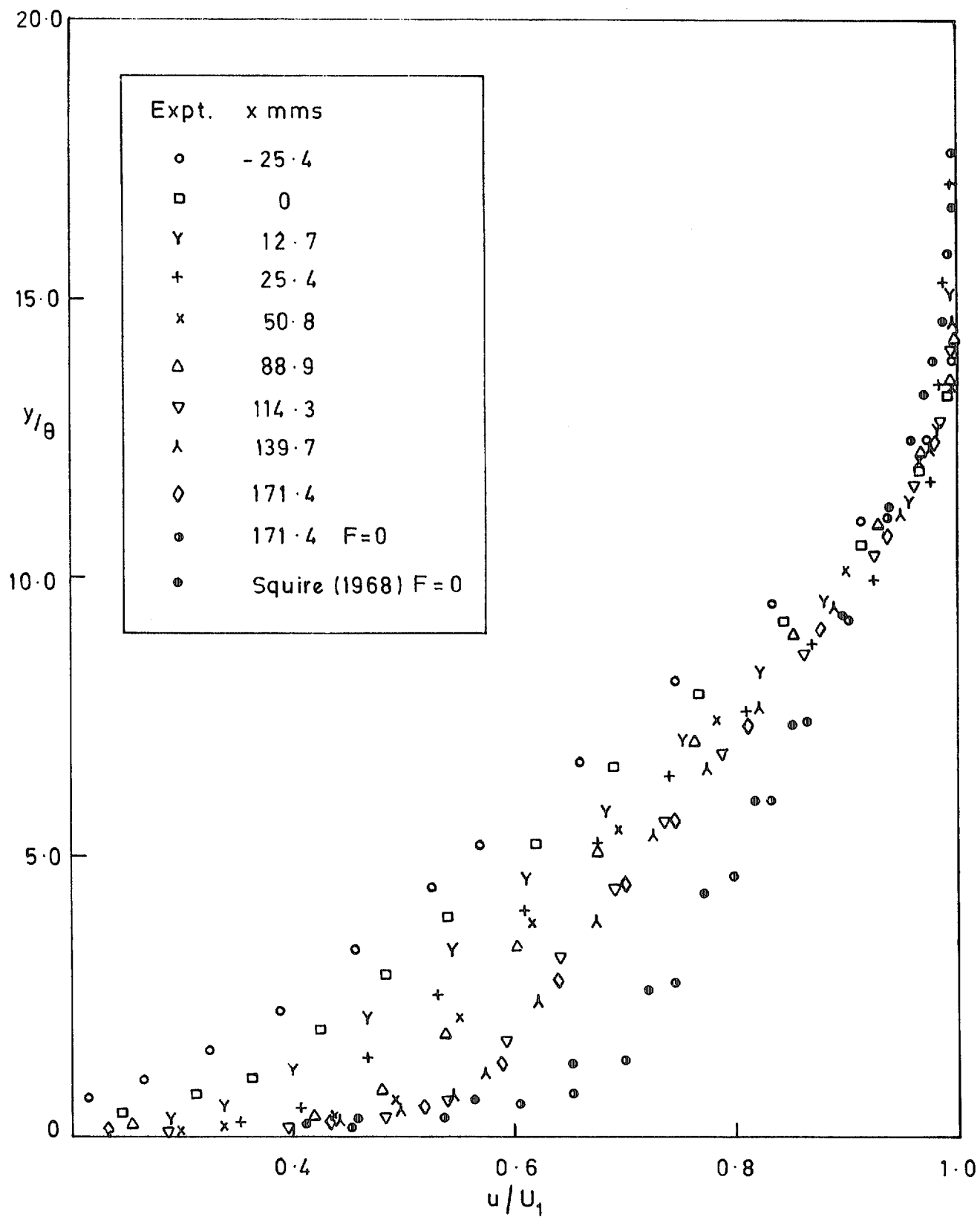
FIG. 31. y/\theta vs u/U_1 ( M = 3.6 ; F = 0.00294 porous-solid).
