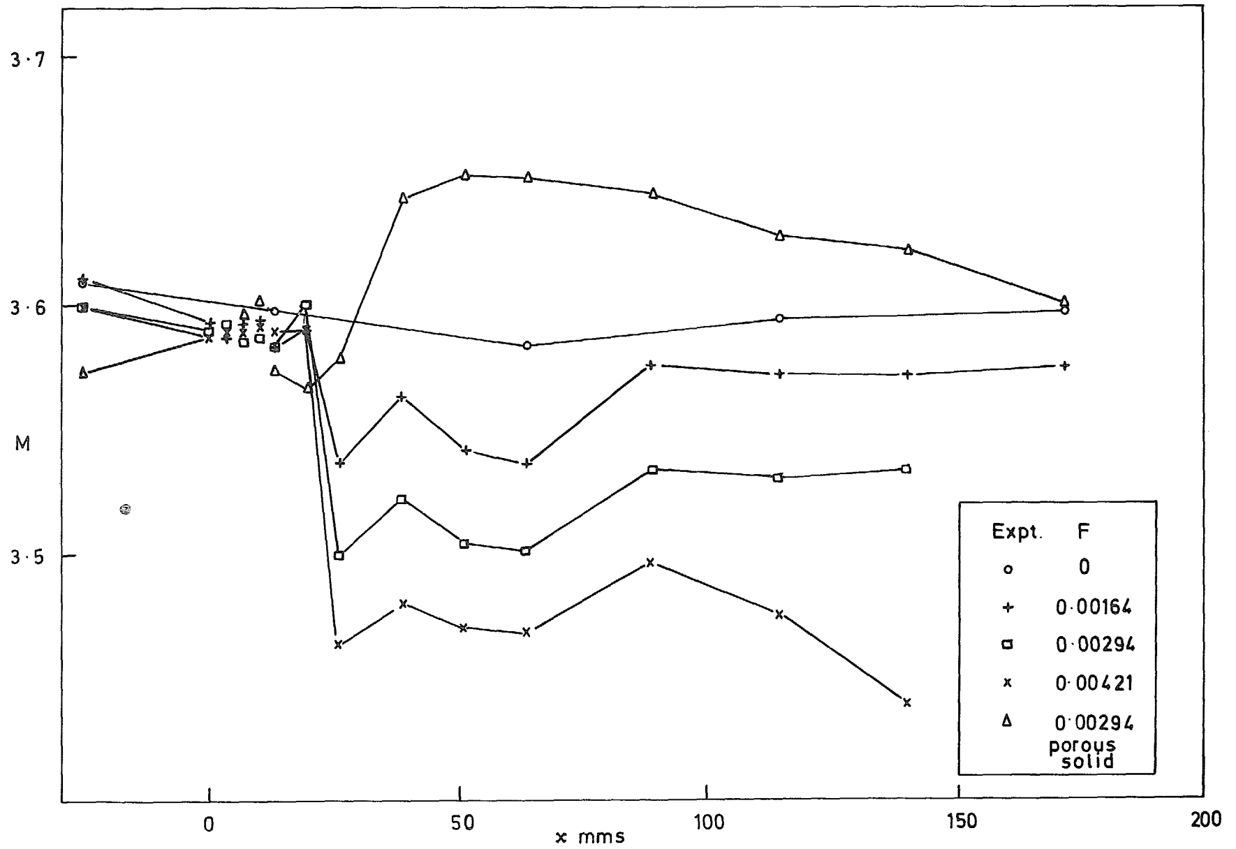
FIG. 9. Mach number distribution.
