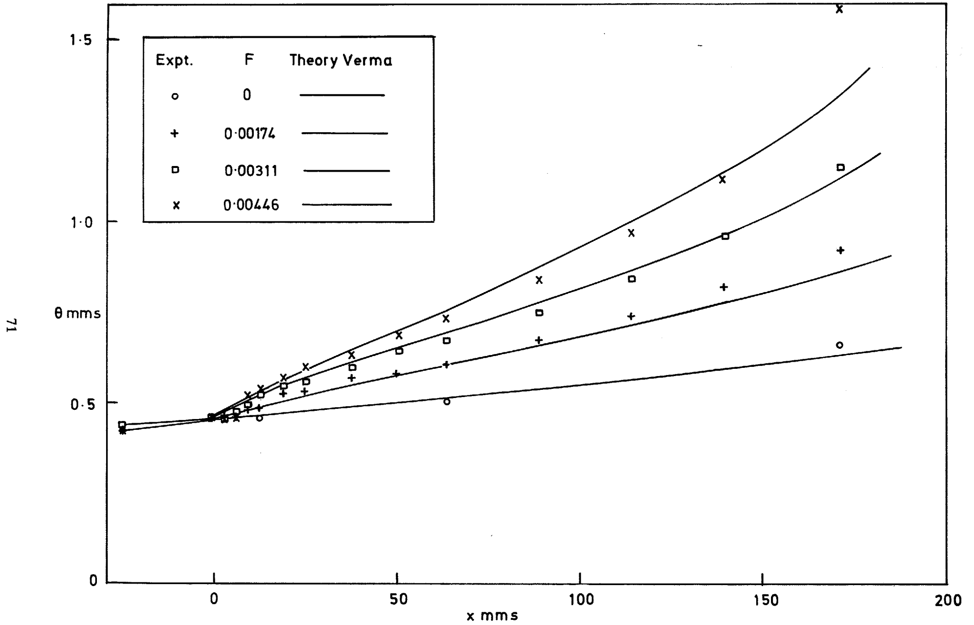
FIG. 24. Momentum thickness development ( M = 1.8 ).
