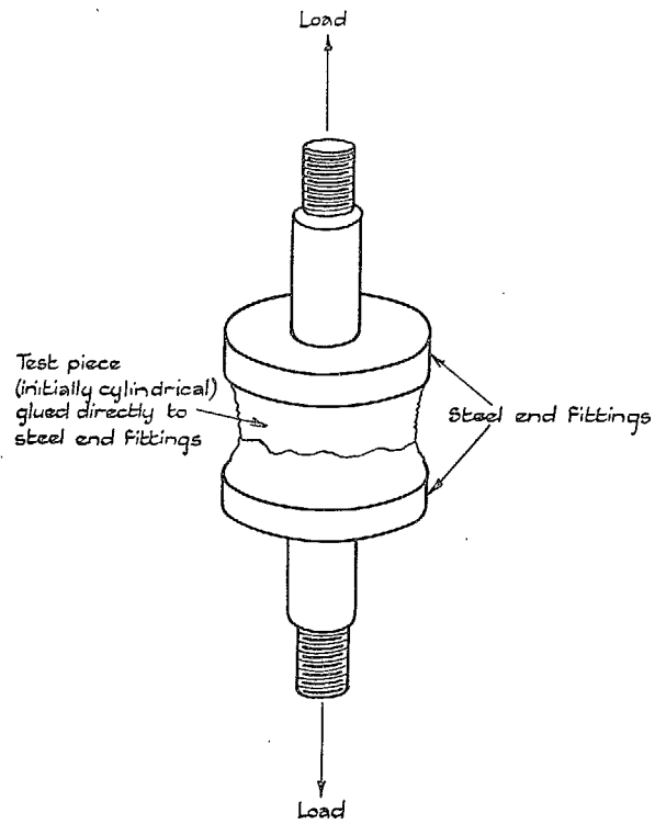
(b) Cross-grain tensile test piece
