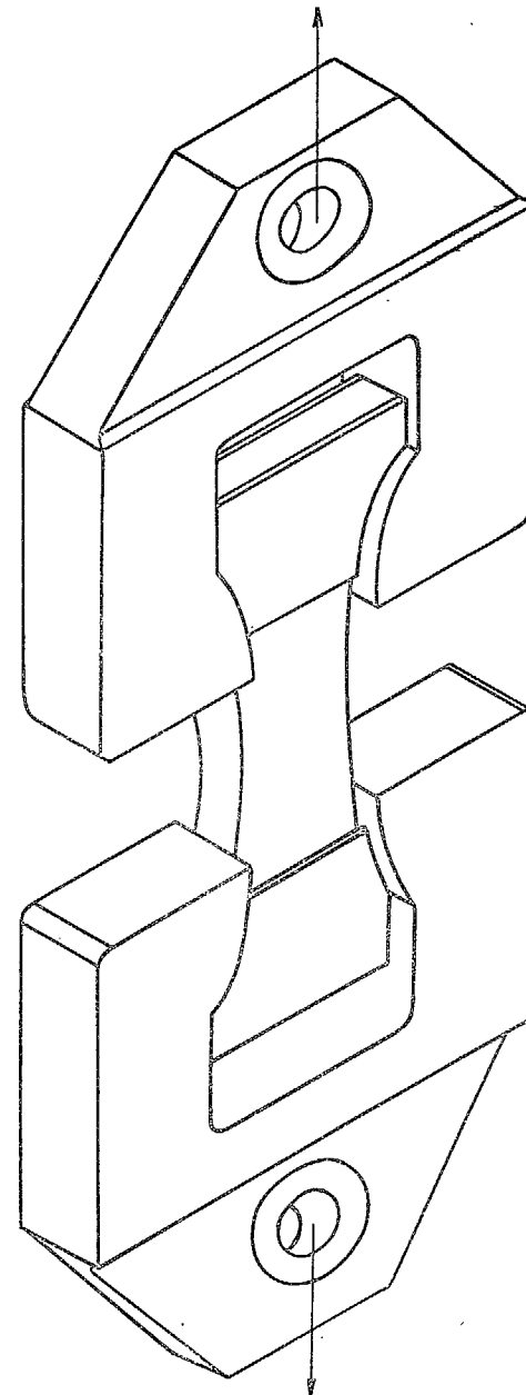
FIG. 2. Dumb-bell type grips used for the 0 deg direction tensile tests.
