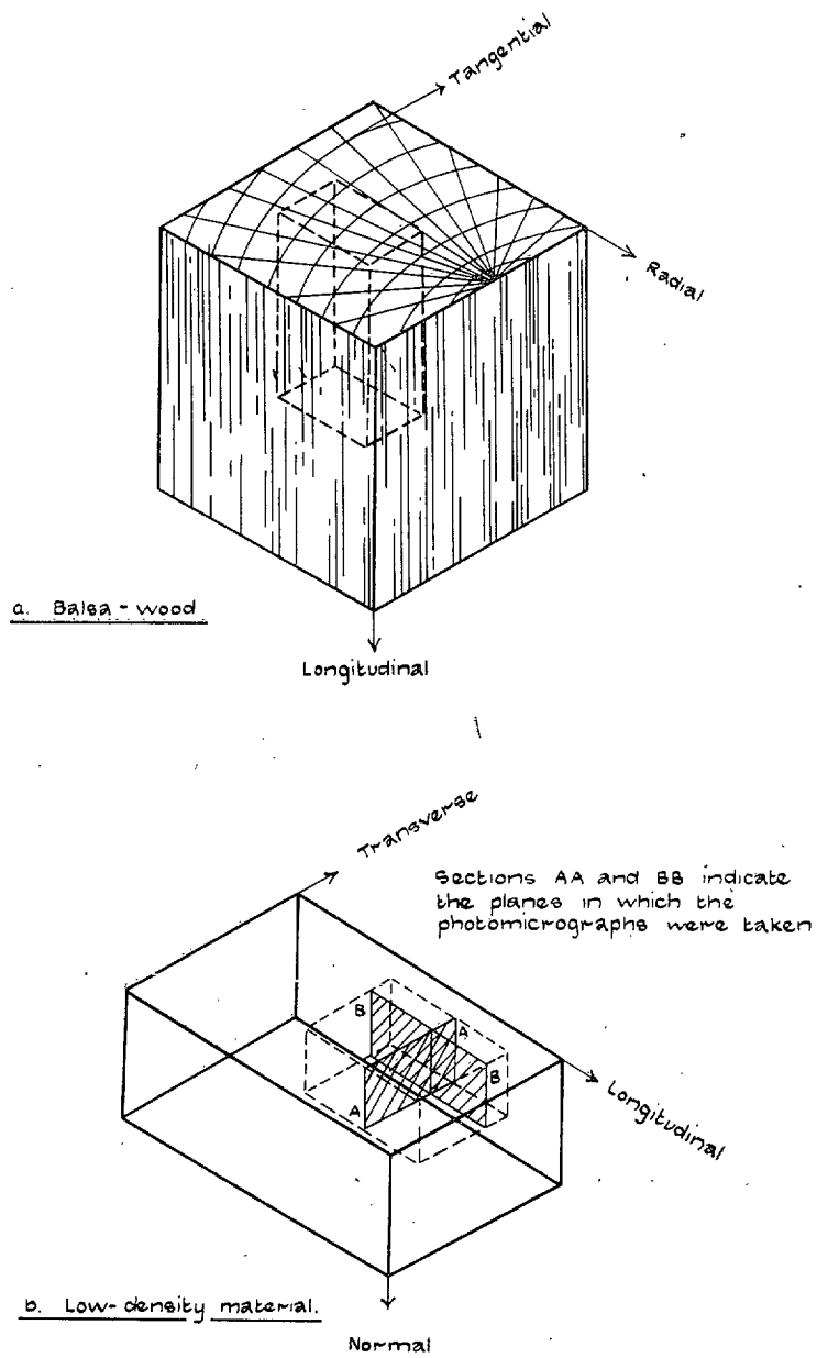
FIG. 1. Sketch showing directions in which test-pieces were cut.
