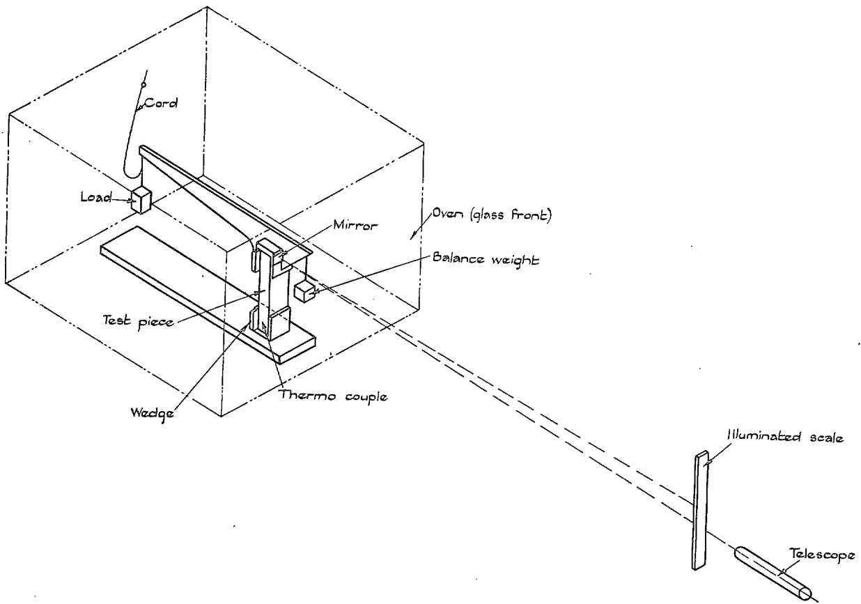
FIG. 3. Arrangement of softening test.
