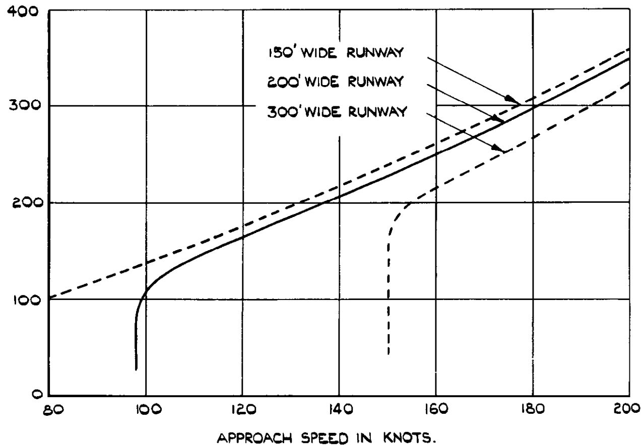
FIG. 5. EFFECT OF APPROACH SPEED AND RUNWAY WIDTH ON HEIGHT AT WHICH THE VISUAL MANOEUVRE MUST START, USING I.L.S. AUTOMATIC APPROACH COUPLER.
